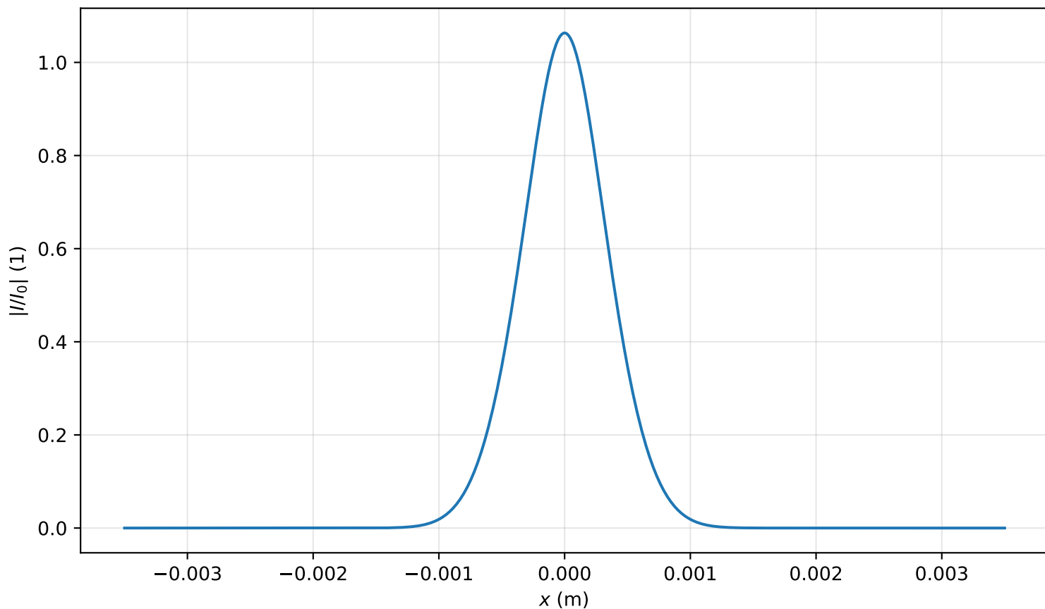
Intensity profile I(x, y = 0, z = 0.398m)/I_0 , P_{in}=0.7P_{cr} , artificial time
